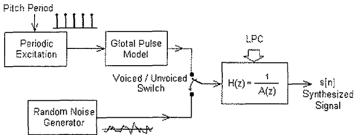
Figure 1: Linear model of speech production.
