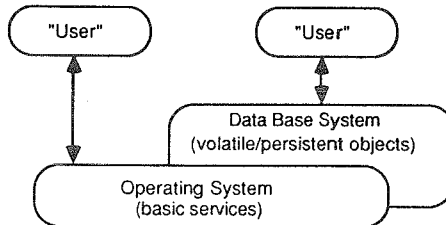
Figure 2. The Operating System and the Data Base System.
