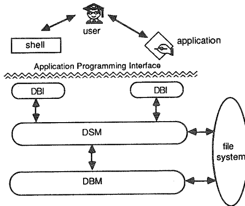
Figure 5. The programs for the data base administration.
