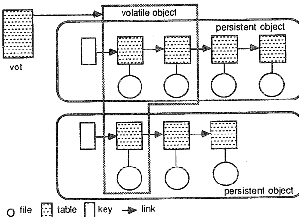
Figure 3. The structure of the data.
