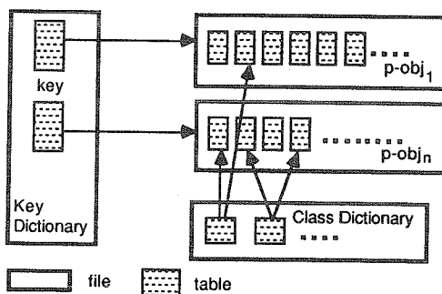
Figure 4. The Key Dictionary and the related structures.
