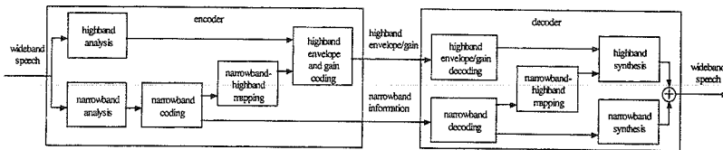
Figure 4. Proposed wideband encoder and decoder based on wideband enhancement
