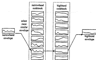
Figure 2. Codebook mapping for highband envelope estimation
