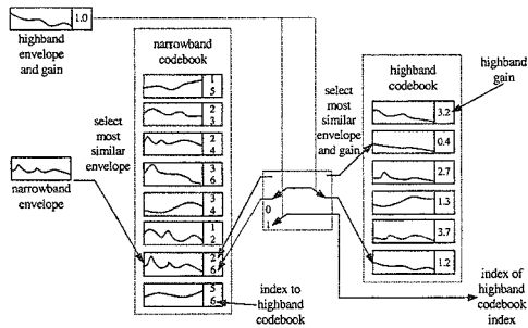
Figure 5. Block diagram example of a classified codebook mapping-based highband envelope and gain encoder using 1 highband bit per frame.
