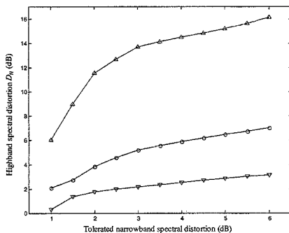
Figure 3. Distribution of continuity-adjusted highband spectral distortion as a function of tolerated (maximum) narrowband spectral distortion. Results are based on around 5 \times 10^6 data points. The percentile contours shown are the 10% ( \nabla ), 50% or median (o), and 90% ( \triangle ). Note that there are relatively few data points at 1 dB tolerated narrowband spectral distortion.
