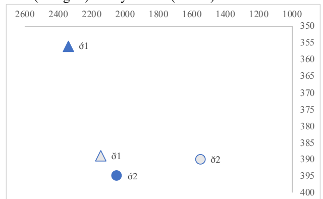
Figure 2: Formant distribution of stressed (darker shades) and unstressed (paler shades) /i/ in syllable 1 (triangles) and syllable 2 (circles).
