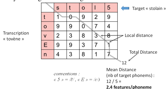
Figure 1: Comparison of 2 phoneme sequences by the Wagner-Fischer algorithm
