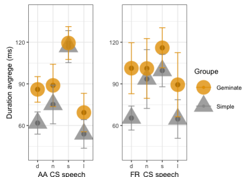
Figure 2: Average duration in (ms) of simple consonants in AA and FR CS speech. Circles: geminate variant selected ( C \rightarrow CC ); triangles: remains simple ( C \rightarrow C ). Error bars give standard deviation.
