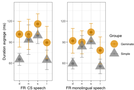
Figure 4: Average duration (ms) of French simple consonants in CS and monolingual speech. Circles: labelled as geminate variant ( C \rightarrow CC ); triangles: ( C \rightarrow C ) Error bars give standard deviation
