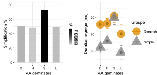
Figure 5: Left: Simplification rates of AA geminates. Right: Average duration (ms) for simple C variants given by triangles ( CC \rightarrow C ); unchanged geminates given by circles ( CC \rightarrow CC variation)
