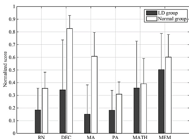
Figure 2: Error chart between LD vs. ND groups in six main tests: Rapid naming (RN), Decoding (DEC), Morphological awareness (MA), Phonological awareness (PA), Mathematics (MATH), and Memory (MEM).
