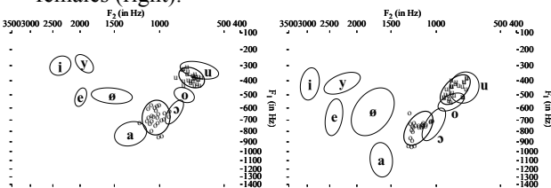
Figure 8: Ellipses of /ou/ of males (left) and females (right).
