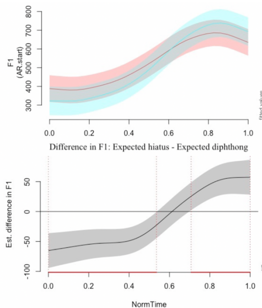
Figure 2. Non-linear smooths (fitted values) and confidence bands (shaded) of F1 formant trajectories by expected category: Diphthong (red) vs Hiatus (blue) (top panel) and difference between the two smooths (bottom panel).
