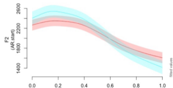
Figure 3. Non-linear smooths (fitted values) and confidence bands (shaded) of F2 formant trajectories by expected category: Diphthong (red) vs Hiatus (blue) (top panel) and difference between the two smooths (bottom panel).
