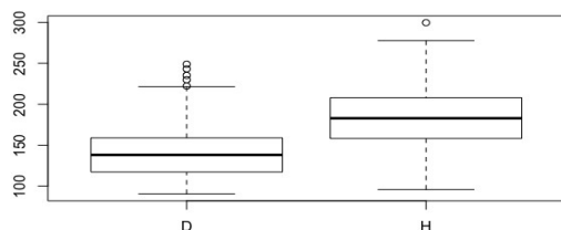
Figure 1. Duration (ms) by expected category: D(diphthong) vs H(iatus)
