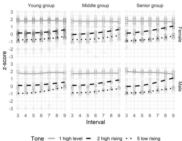
Figure 2: F0 contours of T1, T2 and T5 across age and gender groups, using loess regression.
