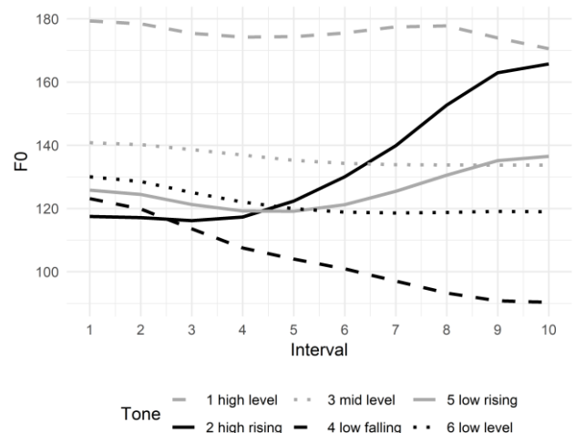
Figure 1: Time-normalised F0 contours of six tones in HK Cantonese, extracted from recordings available on [8].
