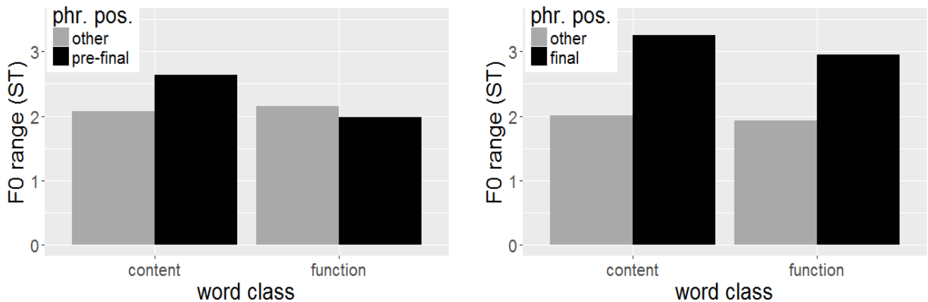
Figure 1: F0 range (ST) of syllables in two-syllable content and function words in pre-final (black, left) and final (black, right) phrase position in comparison with other (grey) positions within the phrase.
