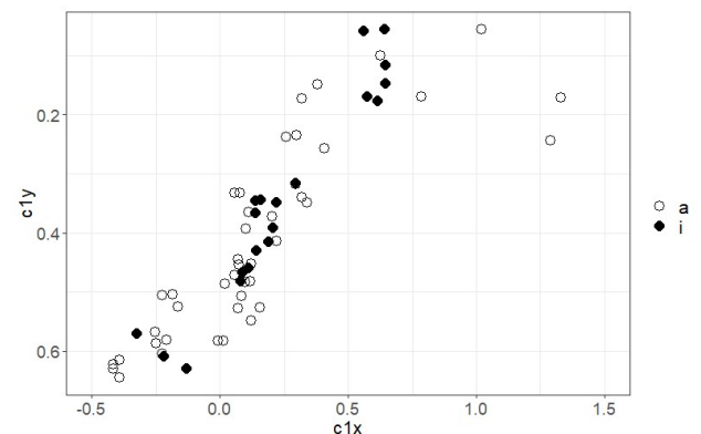
Fig. 3: C1 distribution of medial /N/ as a function of the preceding vowels
