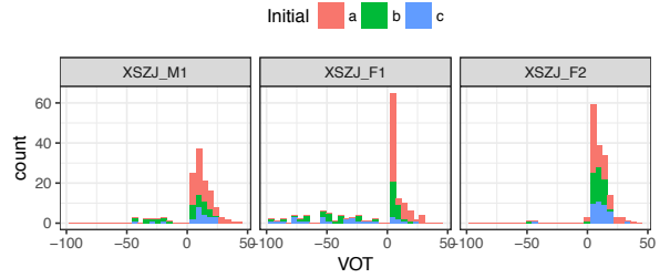
Figure 2: VOT distributions of P_A and P_B by speaker. Blue are MC unaspirated, red are MC aspirated, and green are MC voiced.
