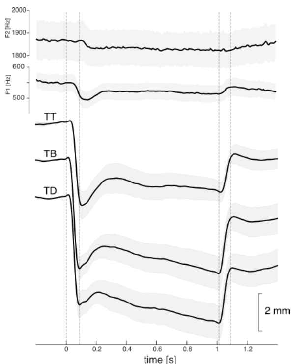
Figure 2: Temporal patterns of the first and second formant frequencies and horizontal displacements of the tongue tip (TT), blade (TB) and dorsum (TD) during the production of voiced /ε/. Time 0 corresponds to the perturbation onset.
