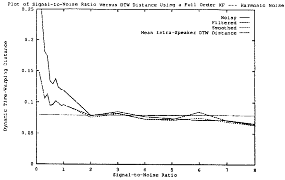
Figure 2: SNR versus DTW distance for the full order Kalman filter/smoothing (Order = 10) with harmonic noise.
