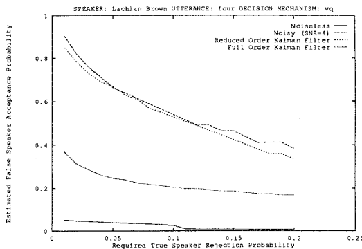
Figure 8: Example 1: Required True Speaker Rejection Rate Versus Estimated False Acceptance Rate — Vector Quantization
