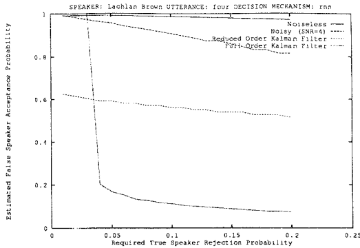
Figure 7: Example 1: Required True Speaker Rejection Rate Versus Estimated False Acceptance Rate — Recurrent Neural Network
