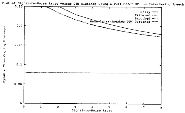
Figure 4: SNR versus DTW distance for the full order Kalman filter/smoothing (Order = 10) with interfering speech.
