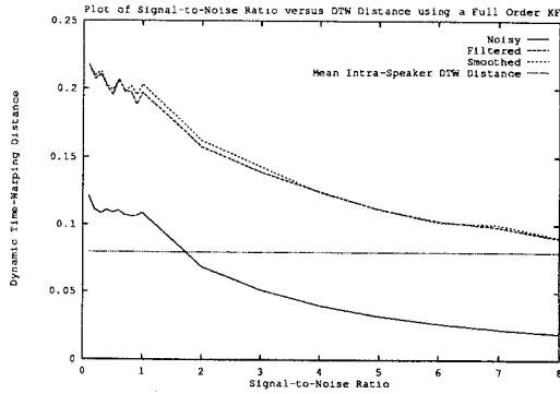
Figure 3: SNR versus DTW distance for the full order Kalman filter/smoothing (Order = 10) with impulsive noise.
