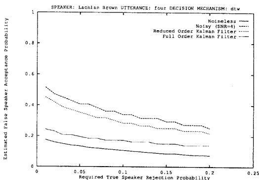
Figure 6: Example 1: Required True Speaker Rejection Rate Versus Estimated False Acceptance Rate — Dynamic Time Warping
